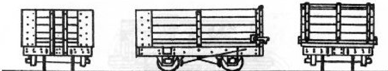
DM36 4-Wheel End Door Open Wagon (based on Vale of Rheidol)
