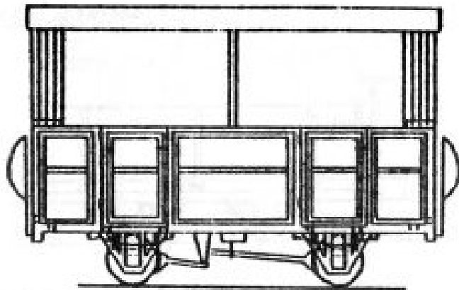
DM34 Open Two Compartment 4-Wheel Coach (based on Vale of Rheidol/Glyn Valley practice)
