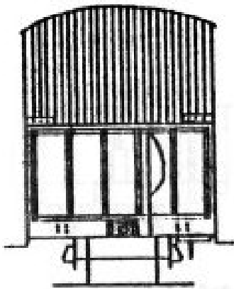
DM34 Open Two Compartment 4-Wheel Coach (based on Vale of Rheidol/Glyn Valley practice)
