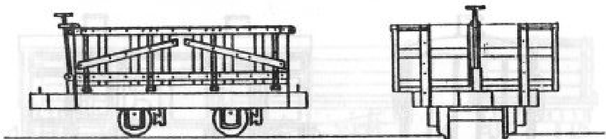
DN32 Hudson 4-Wheel Wooden Bodied Drop Sided Open Wagon
