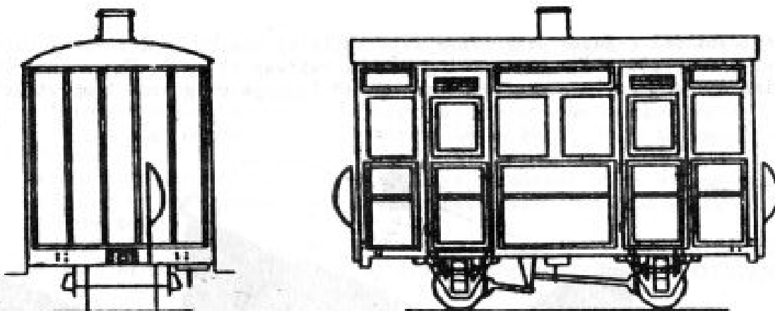
DM29 Two Compartment 4-Wheel Coach (based on Vale of Rheidol/Glyn Valley practice)
