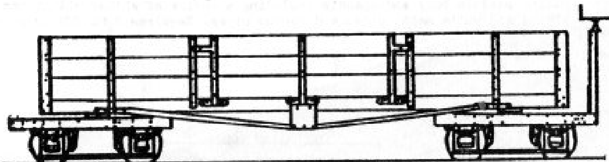
DM30 W.W.1 War Dept. Modified Class E Dropdoor Bogie Open Wagon (ex Ashover Light Railway)
