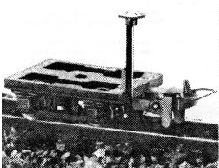
DM20 W.W.1 War Dept. Bogies (pair)
