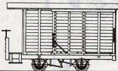
R 809 4w Van with Brake Platform
