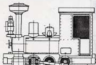
R211 鉄連型SL・0-6-0T KRAUSS
