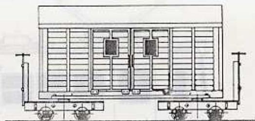
R810 木曾E型貨車・KISO BOX CAR
